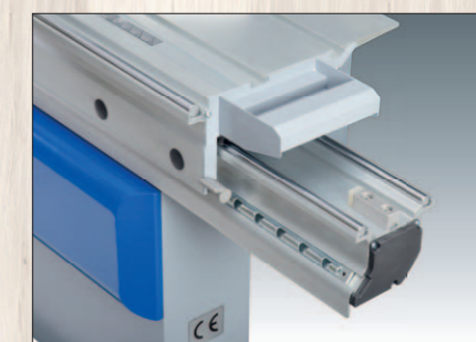
S New sliding table CV 400 T on steel bars
